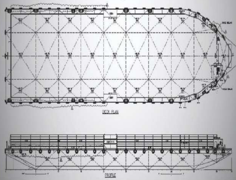
General Arrangement
